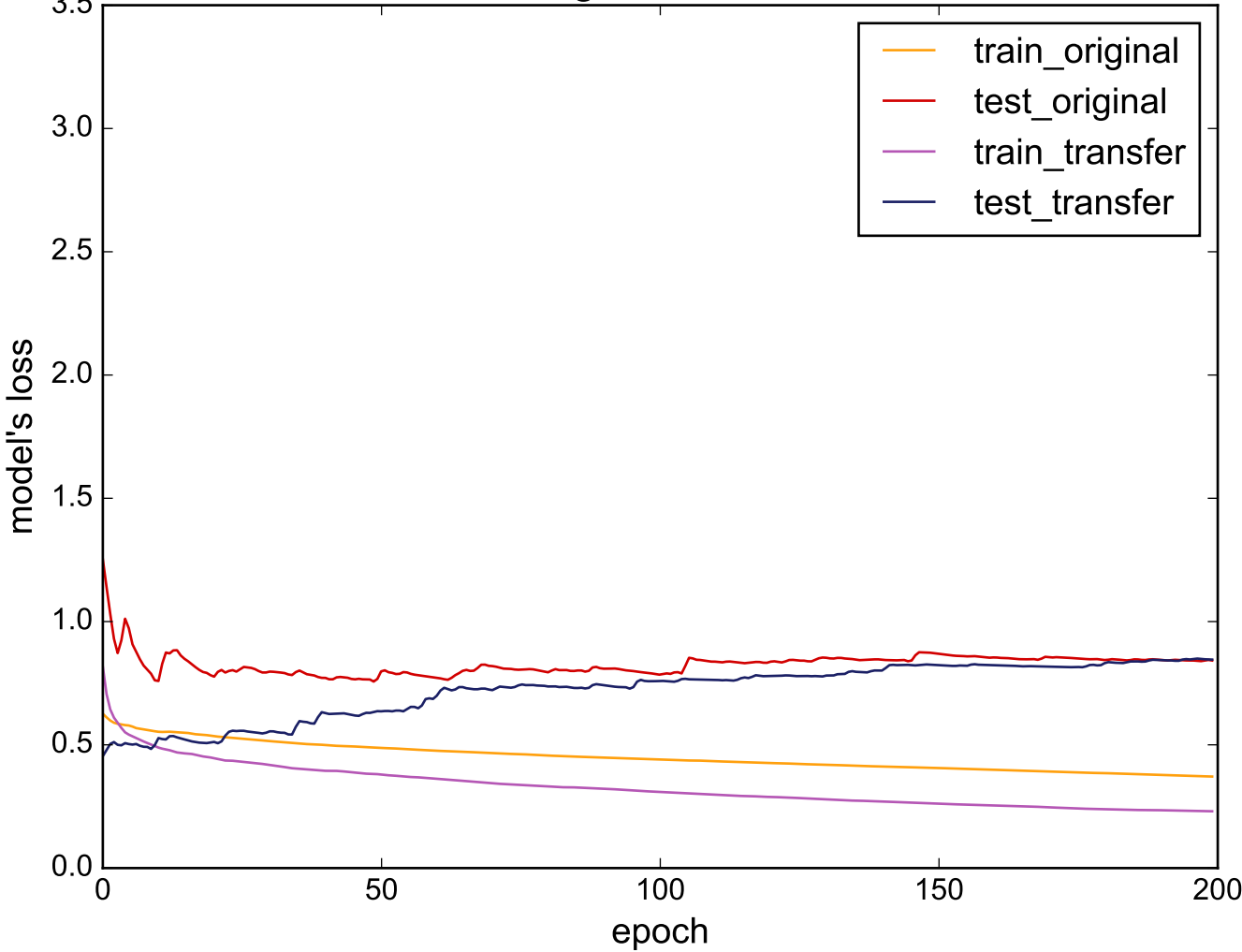
Source: Phoneme - Target: DistalPhalanxOutlineCorrect
