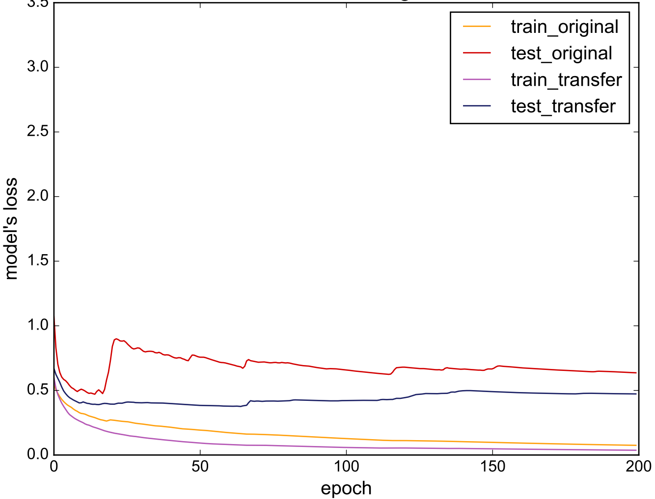
Source: Phoneme - Target: ECG200
