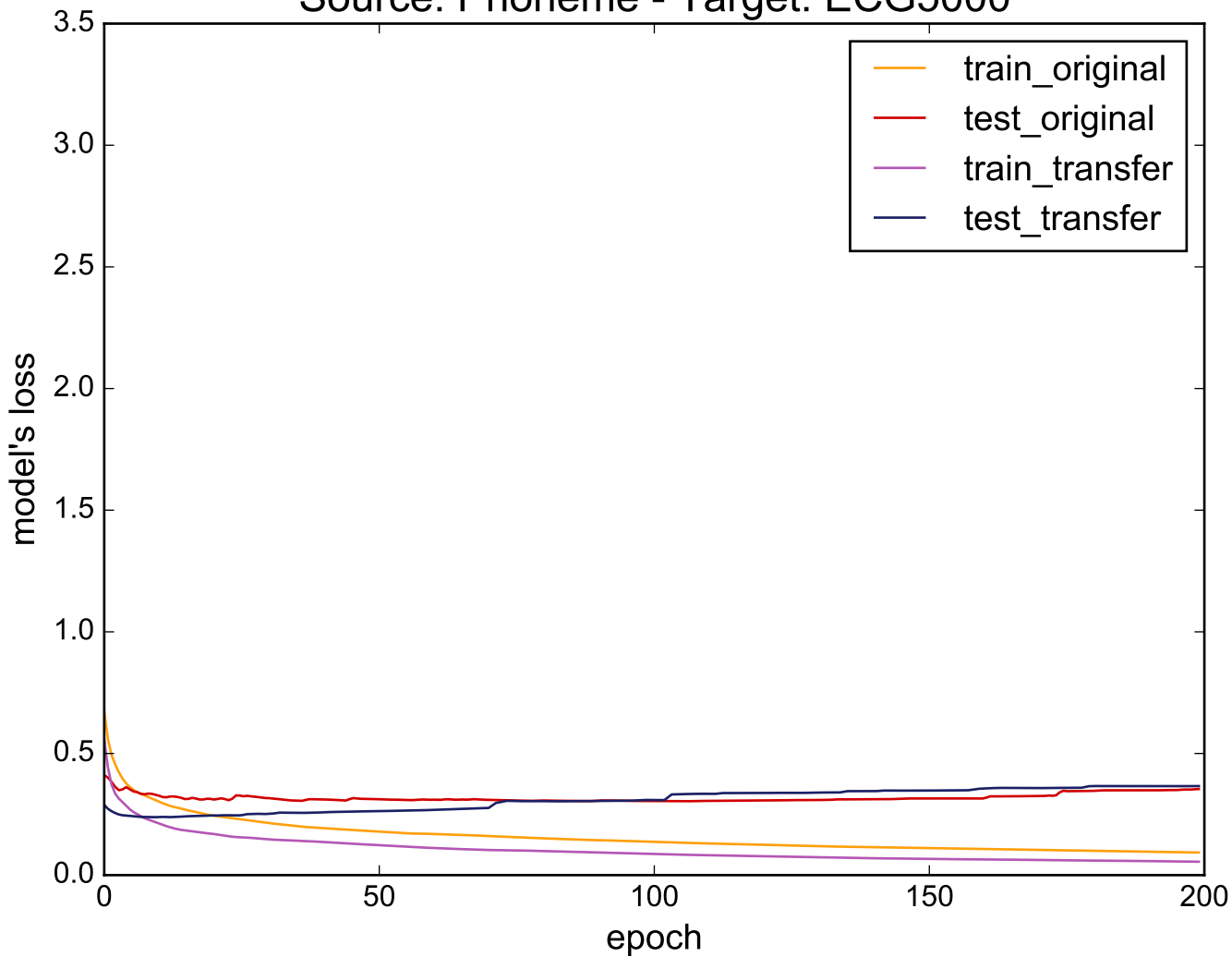
Source: Phoneme - Target: ECG5000
