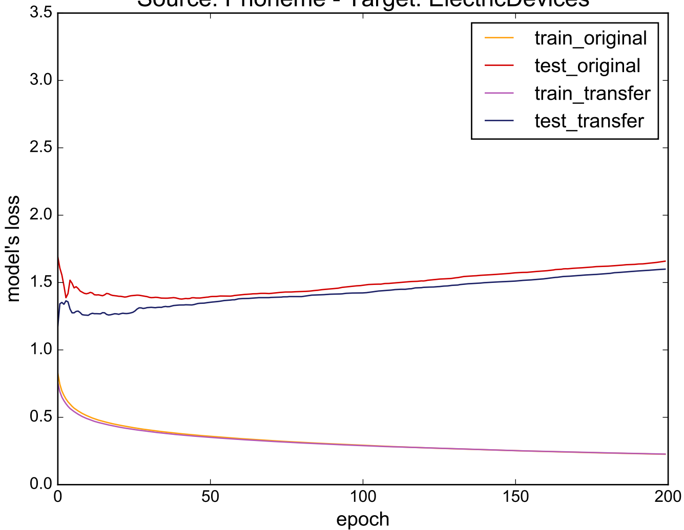
Source: Phoneme - Target: ElectricDevices
