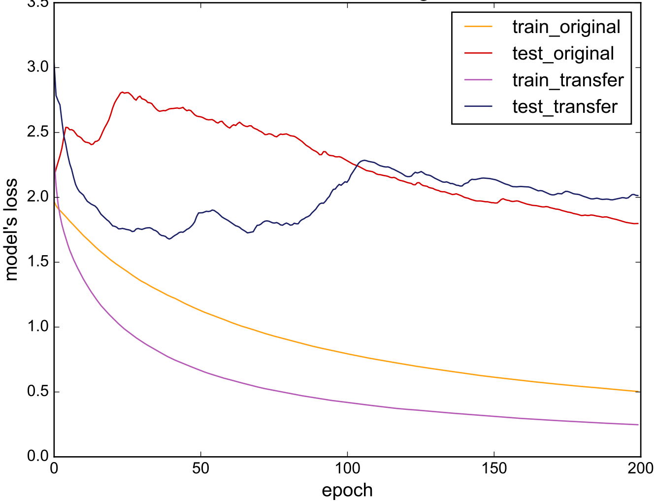
Source: Phoneme - Target: FISH
