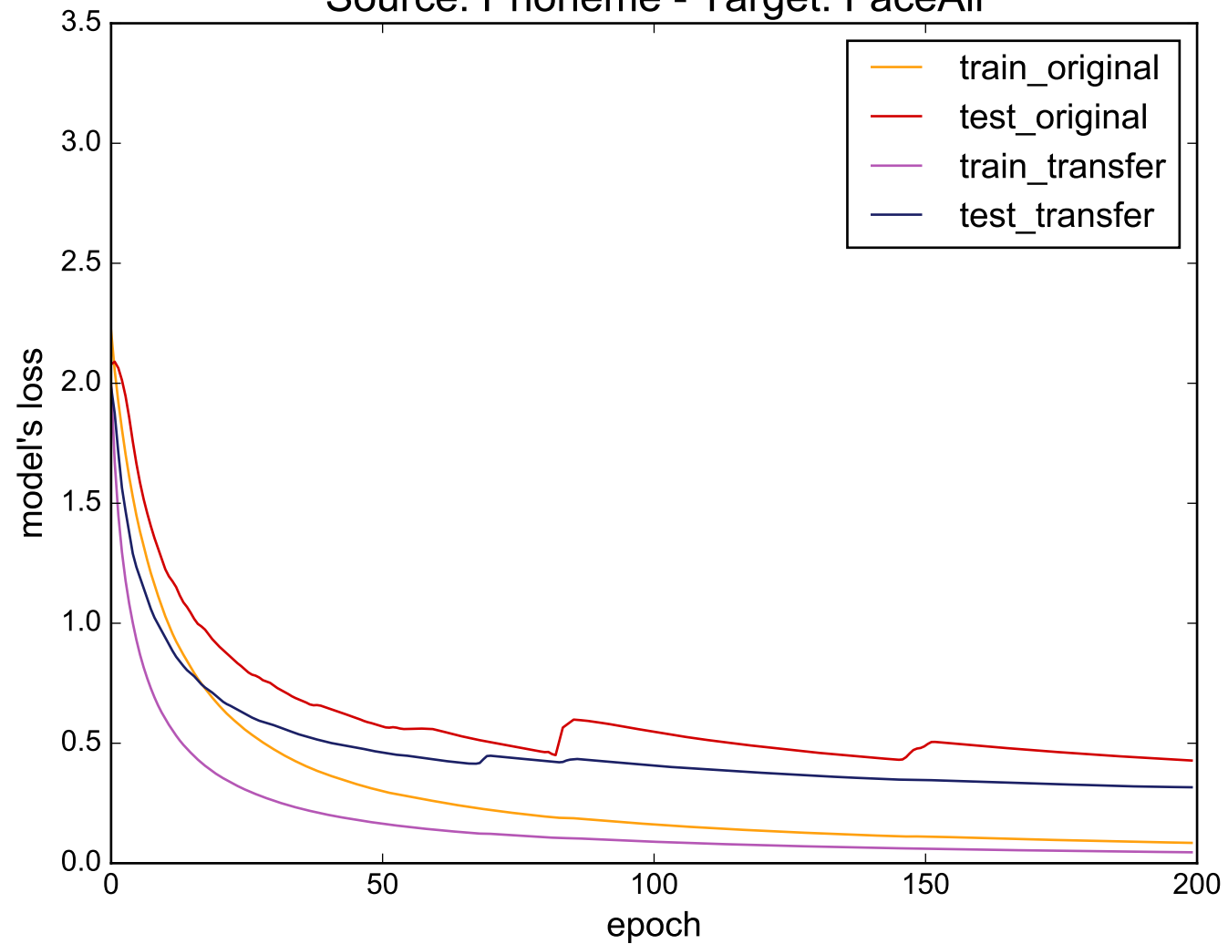
Source: Phoneme - Target: FaceAll
