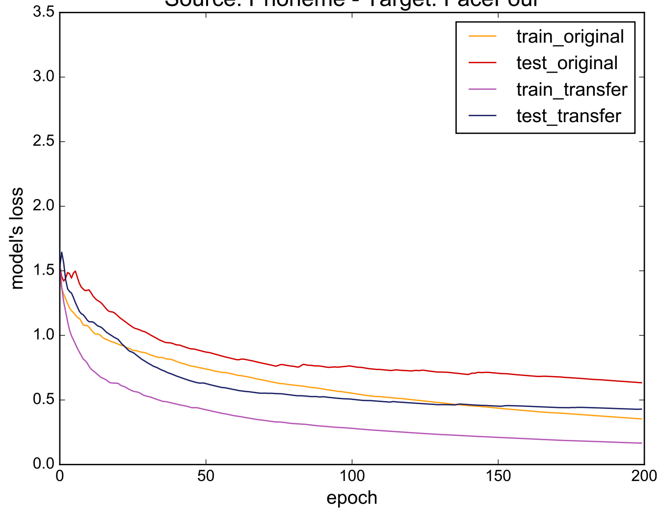
Source: Phoneme - Target: FaceFour
