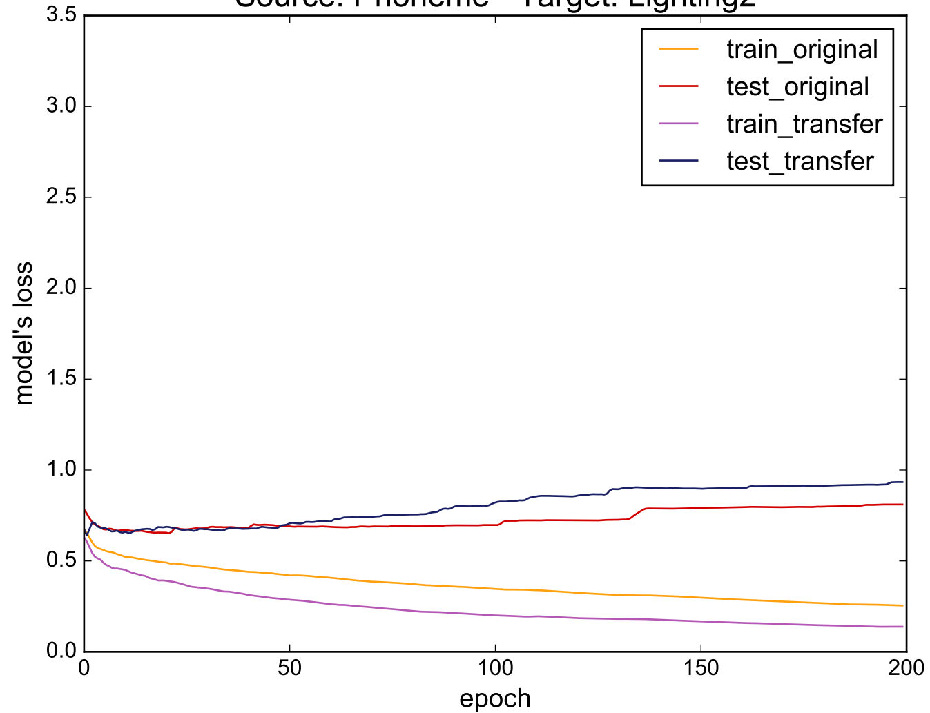
Source: Phoneme - Target: Lighting2
