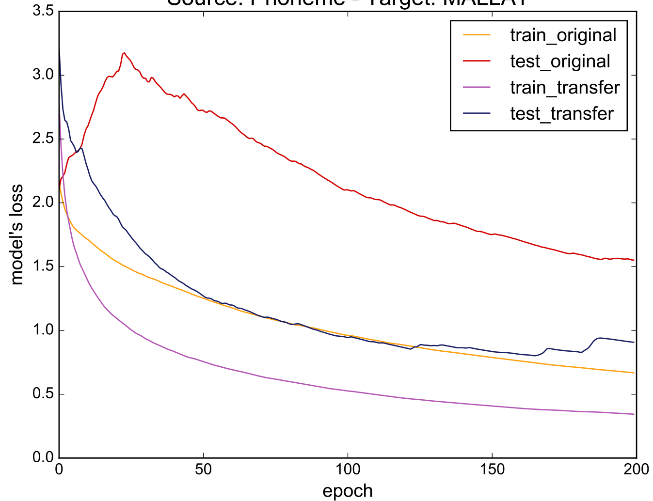
Source: Phoneme - Target: MALLAT
