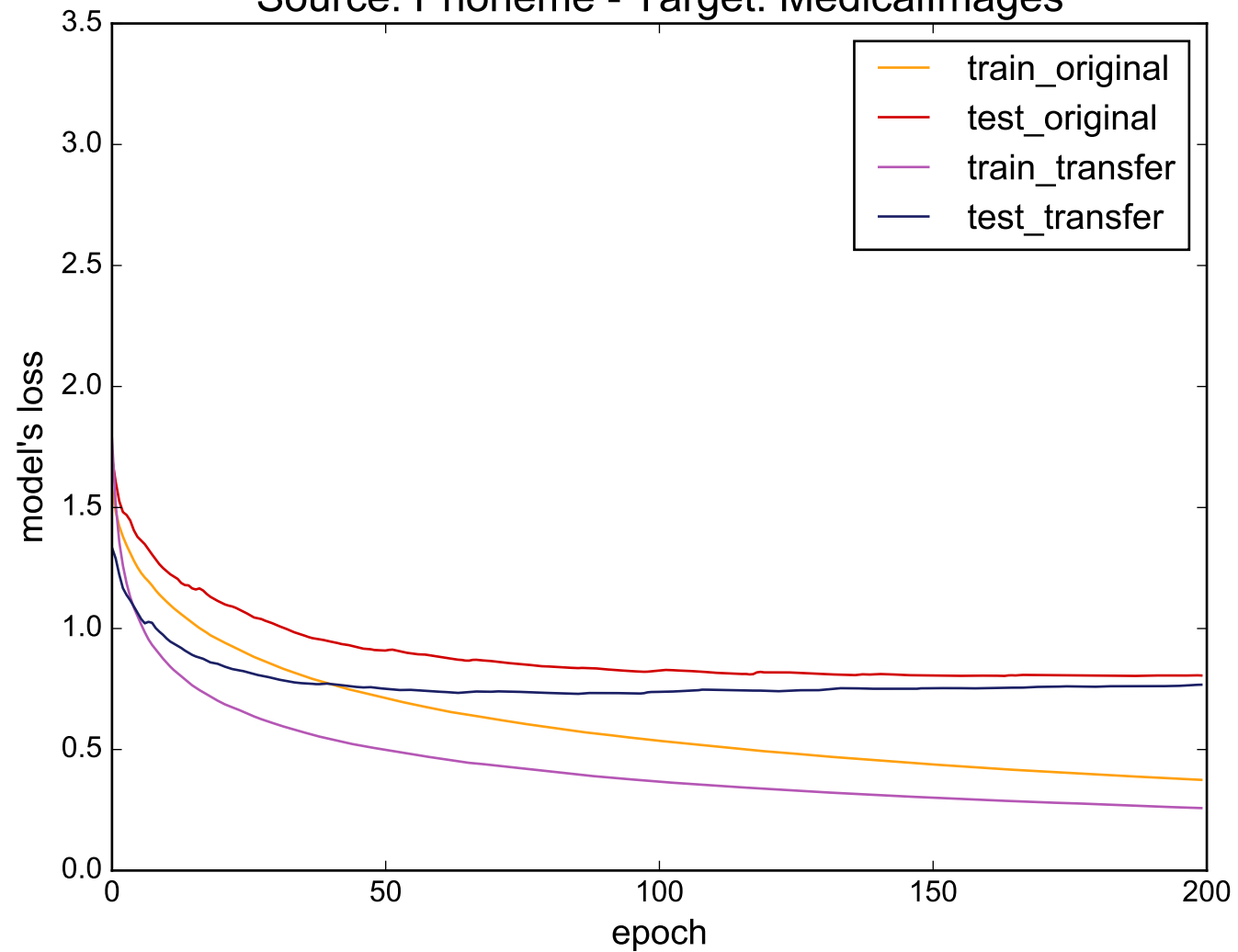
Source: Phoneme - Target: MedicalImages
