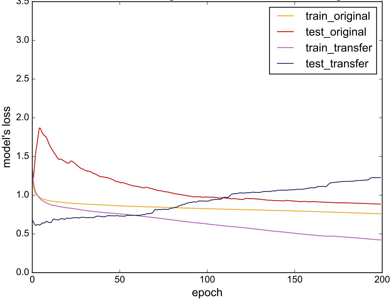
Source: Phoneme - Target: MiddlePhalanxOutlineAgeGroup
