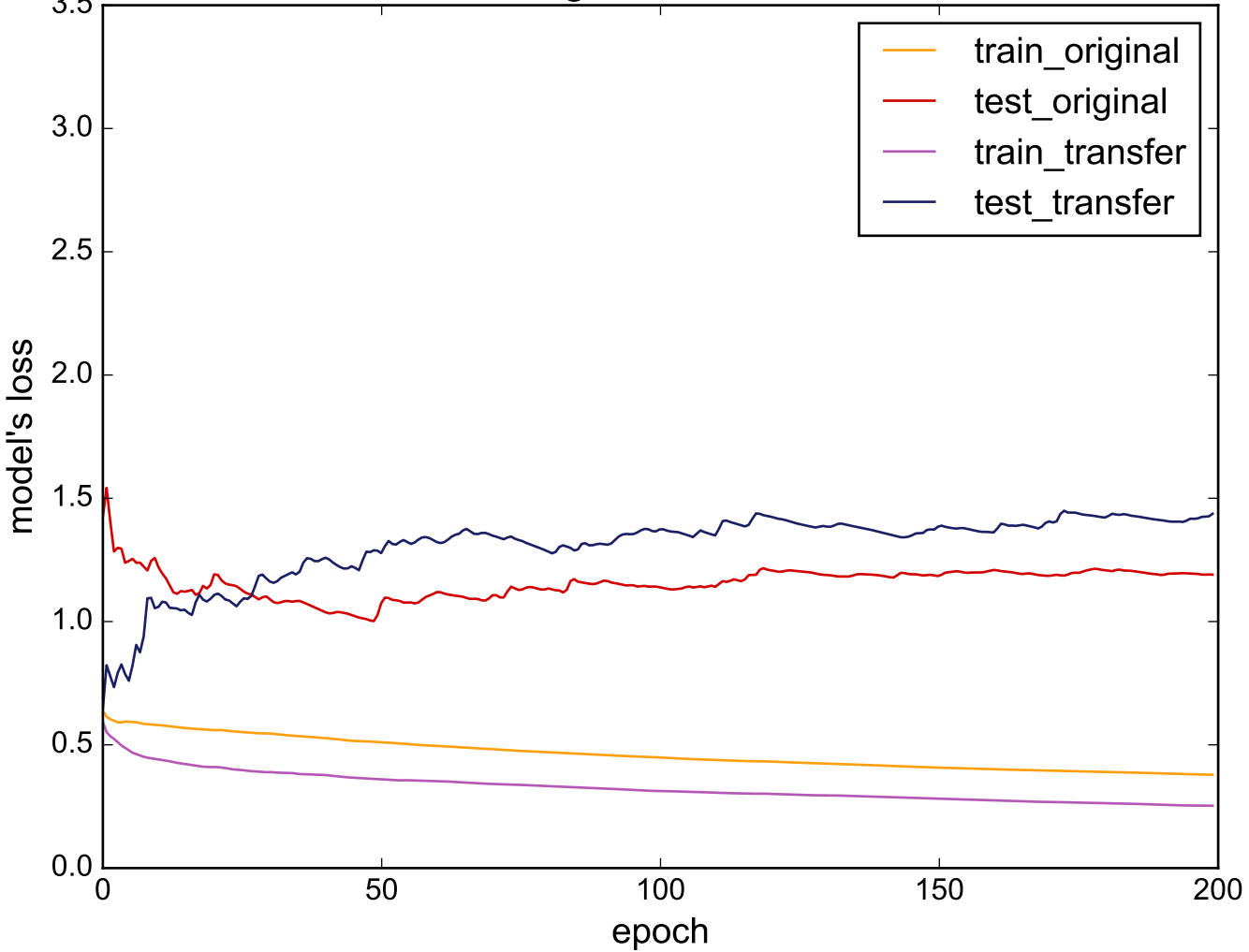
Source: Phoneme - Target: MiddlePhalanxOutlineCorrect
