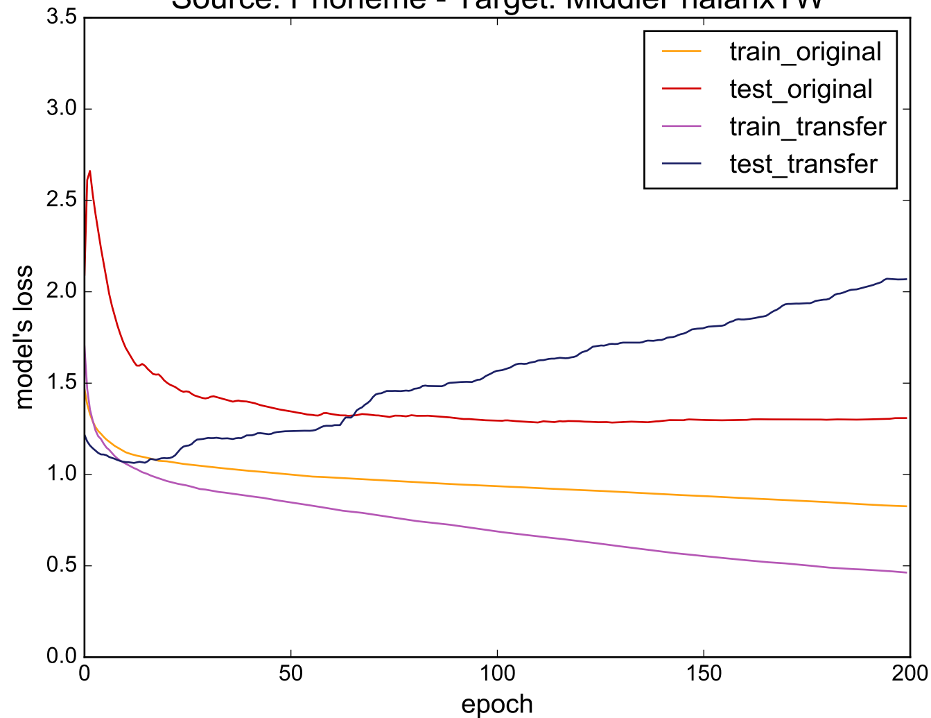
Source: Phoneme - Target: MiddlePhalanxTW
