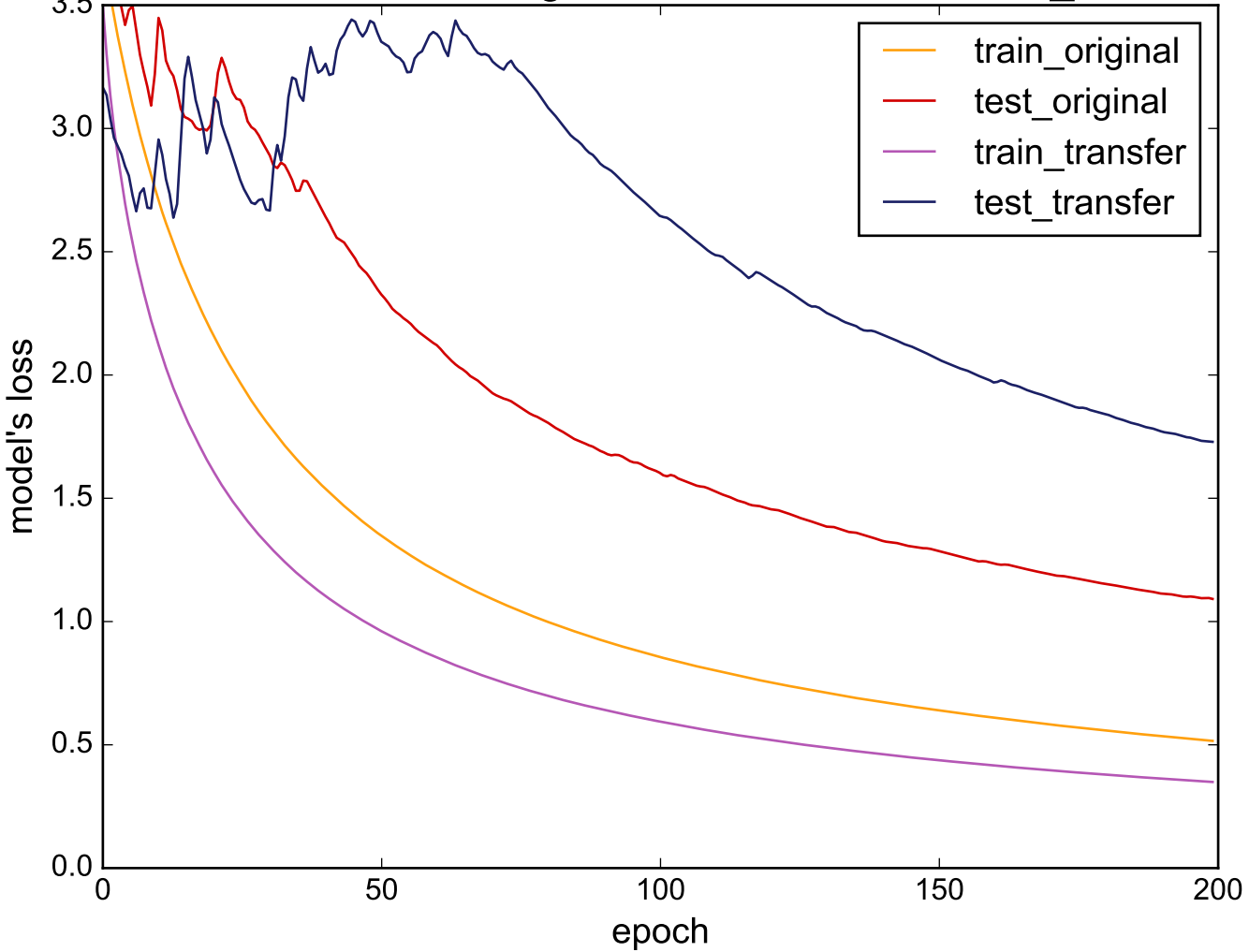
Source: Phoneme - Target: NonInvasiveFetalECG_Thorax1
