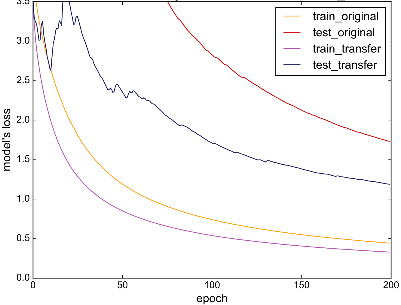
Source: Phoneme - Target: NonInvasiveFetalECG_Thorax2
