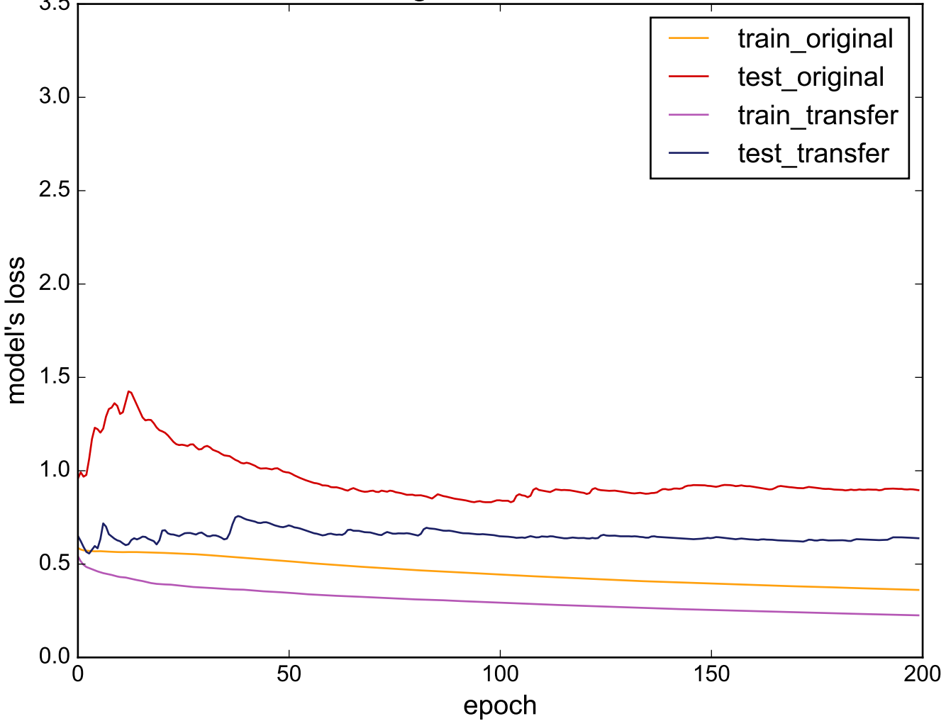
Source: Phoneme - Target: ProximalPhalanxOutlineCorrect
