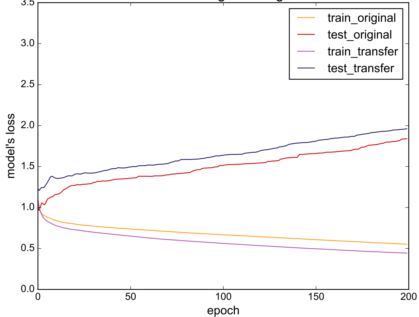
Source: Phoneme - Target: RefrigerationDevices
