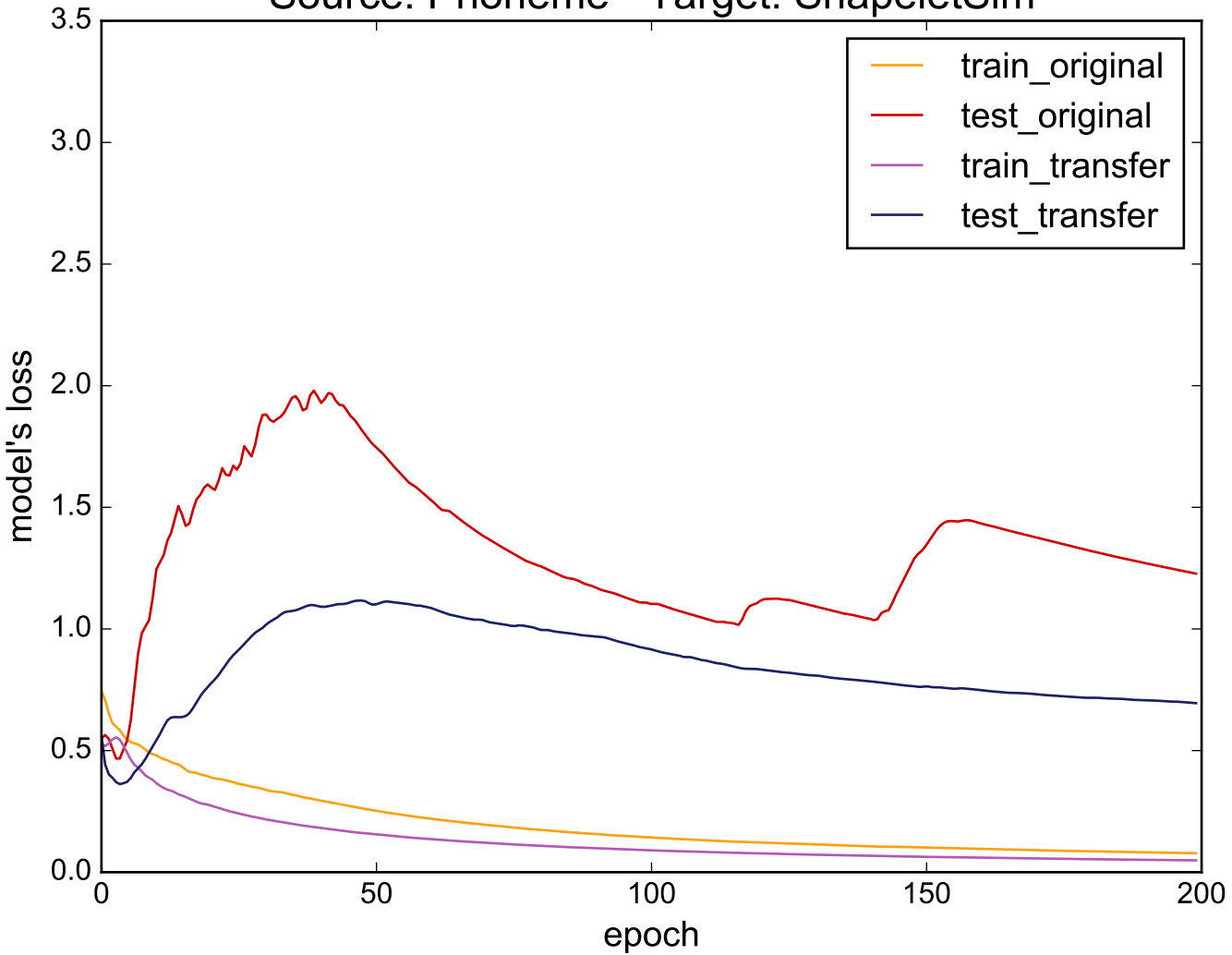
Source: Phoneme - Target: ShapeletSim
