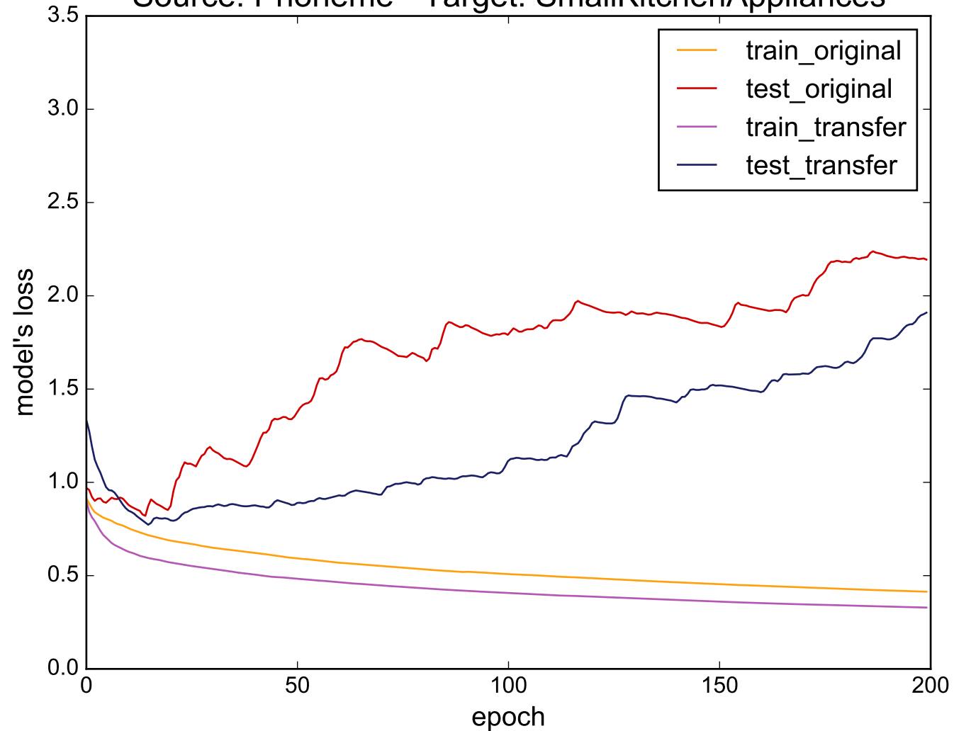
Source: Phoneme - Target: SmallKitchenAppliances
