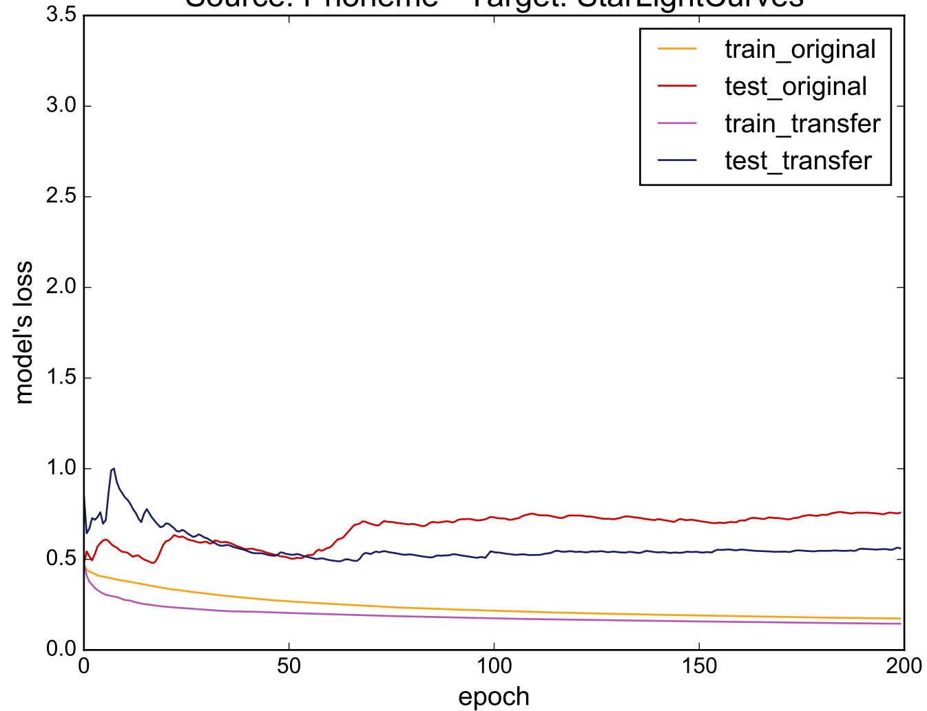
Source: Phoneme - Target: StarLightCurves
