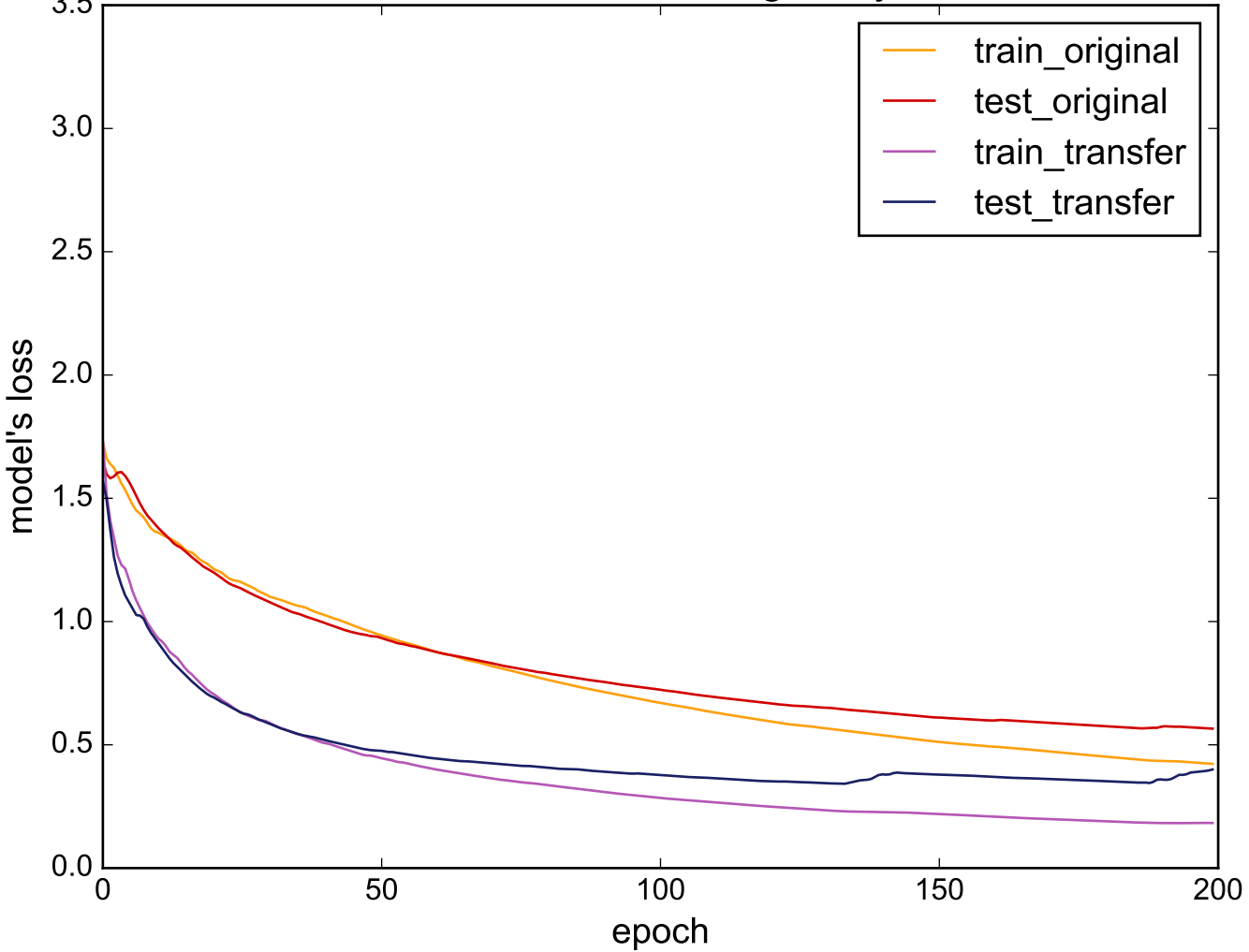
Source: Phoneme - Target: Symbols
