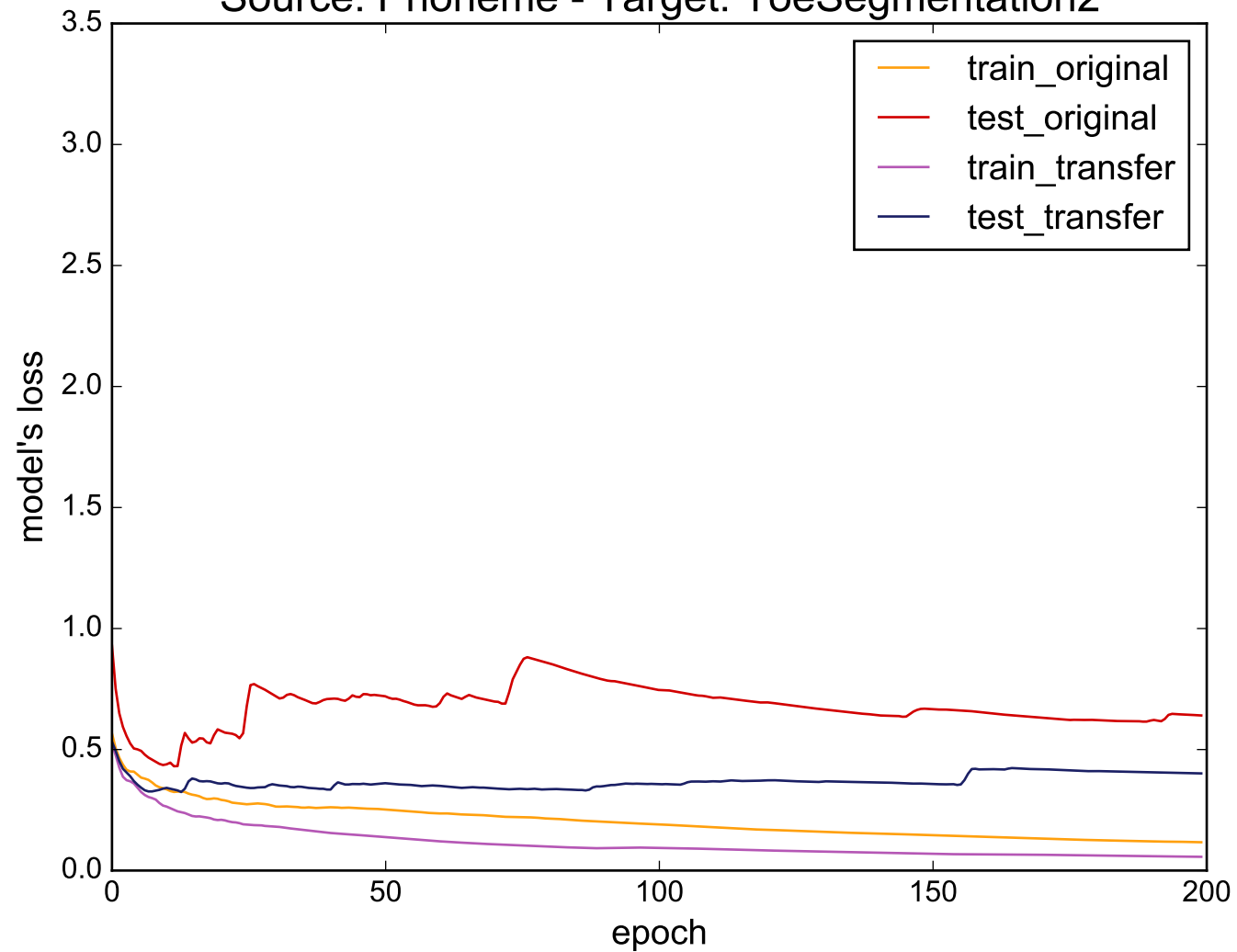
Source: Phoneme - Target: ToeSegmentation2
