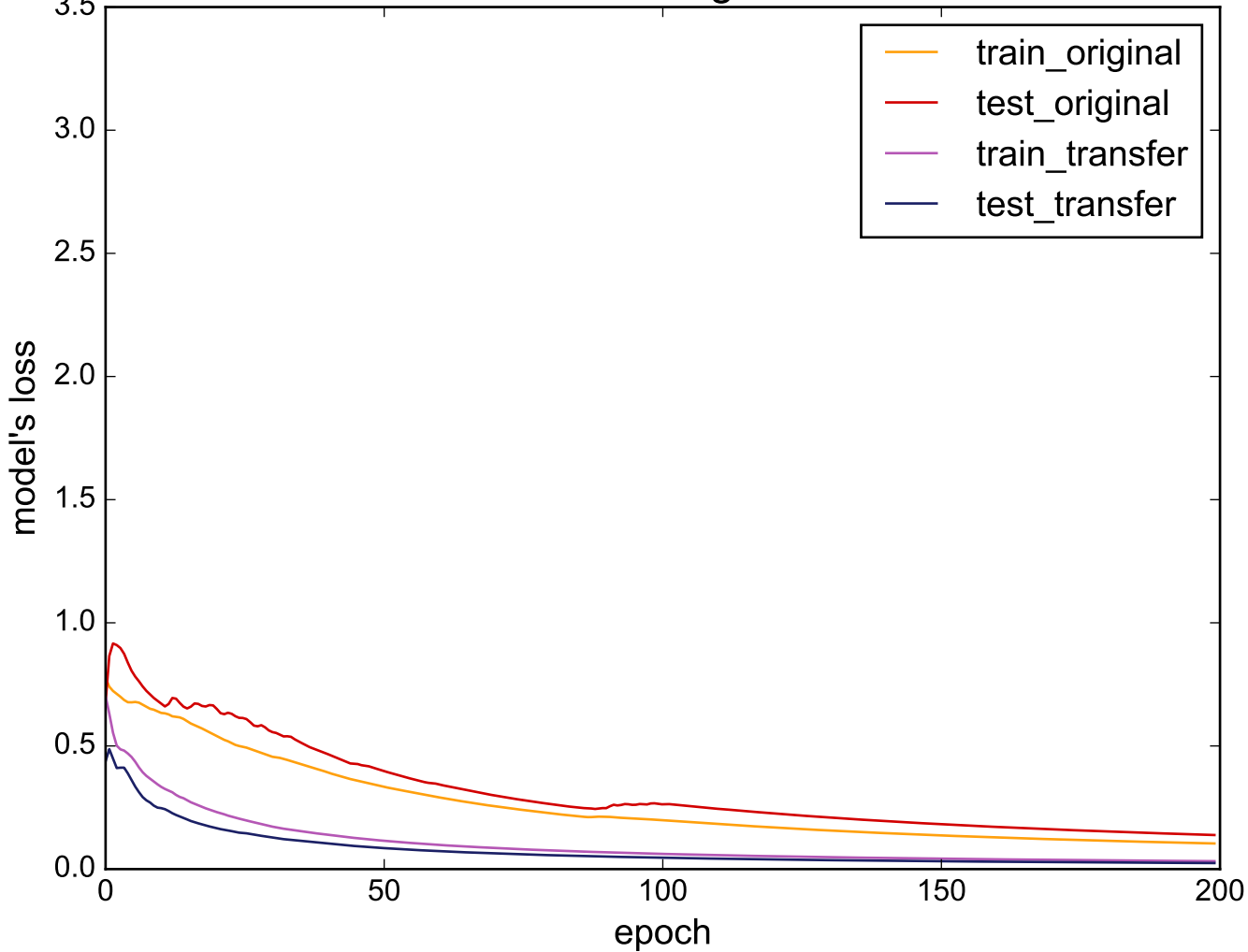
Source: Phoneme - Target: TwoLeadECG
