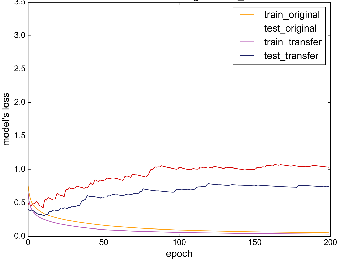
Source: Phoneme - Target: Two_Patterns
