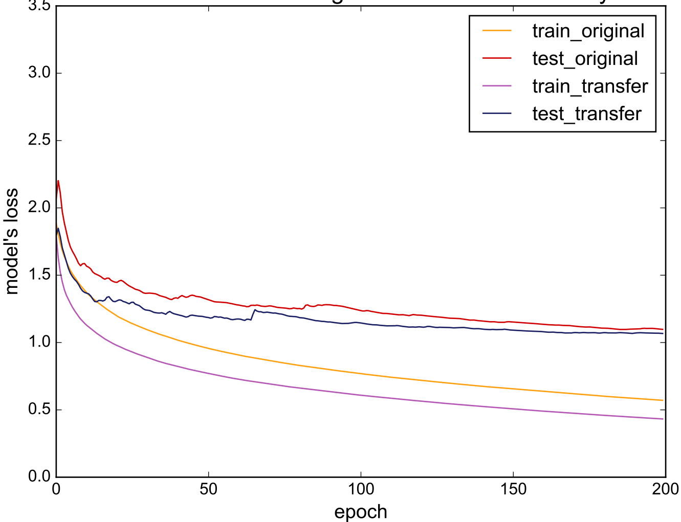
Source: Phoneme - Target: UWaveGestureLibraryAll
