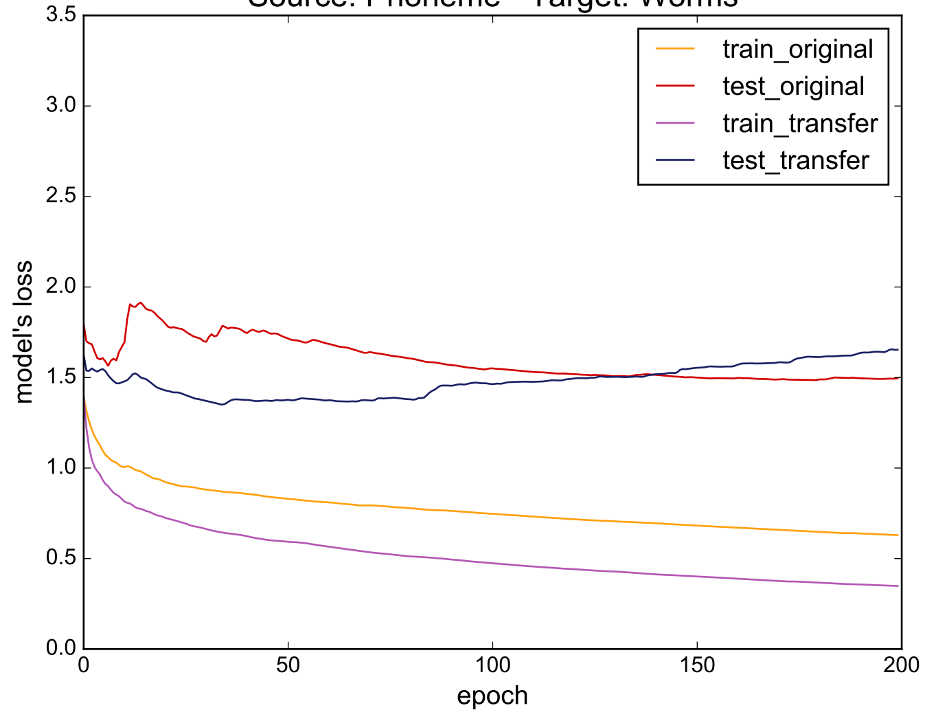
Source: Phoneme - Target: Worms
