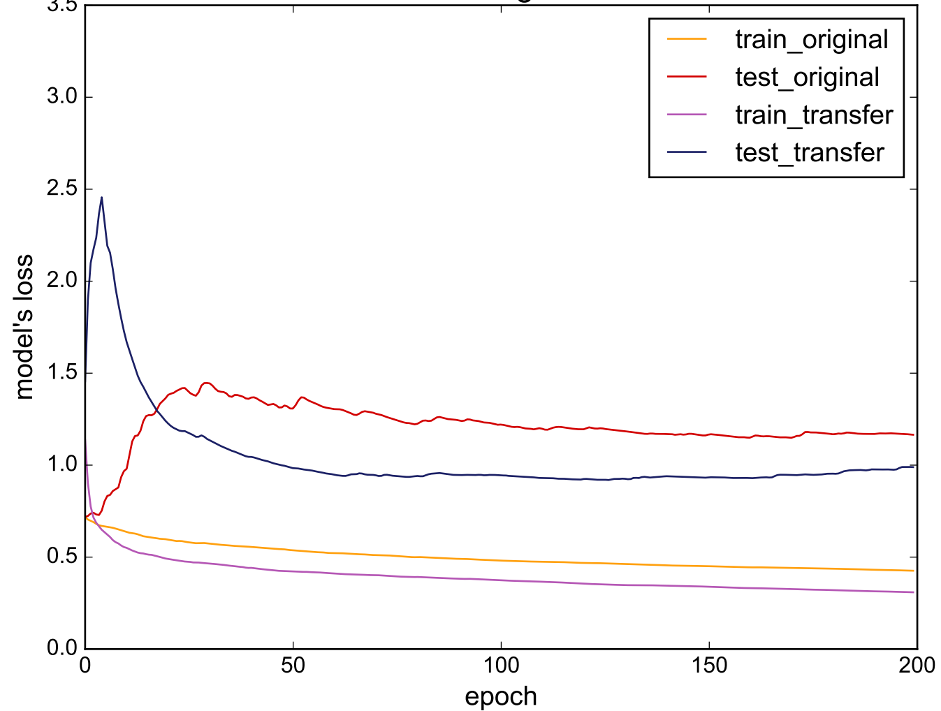
Source: Phoneme - Target: WormsTwoClass
