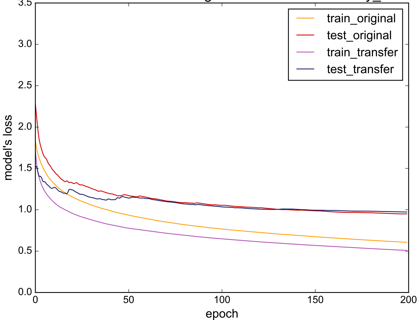
Source: Phoneme - Target: uWaveGestureLibrary_X
