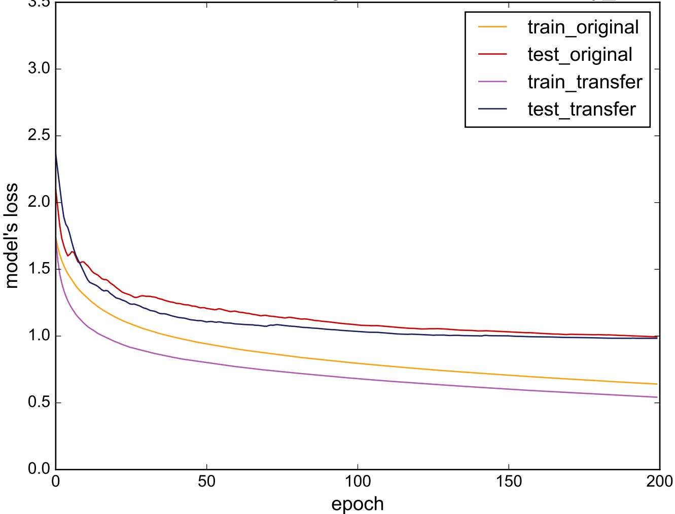
Source: Phoneme - Target: uWaveGestureLibrary_Z
