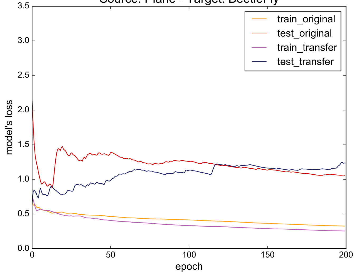
Source: Plane - Target: BeetleFly
