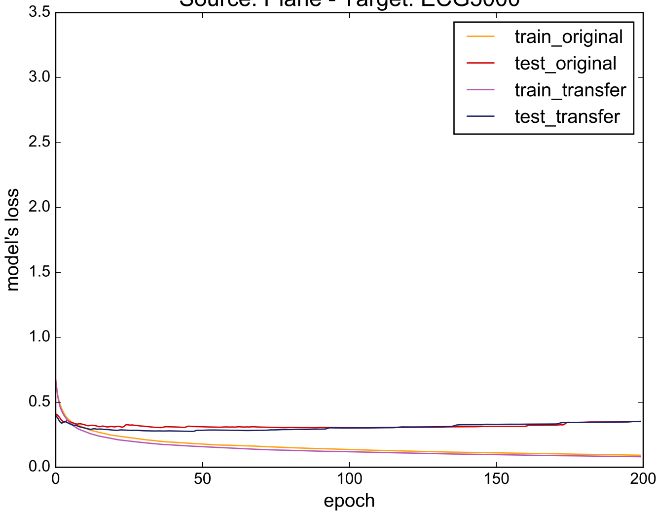
Source: Plane - Target: ECG5000
