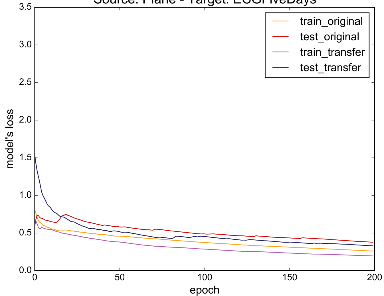
Source: Plane - Target: ECGFiveDays
