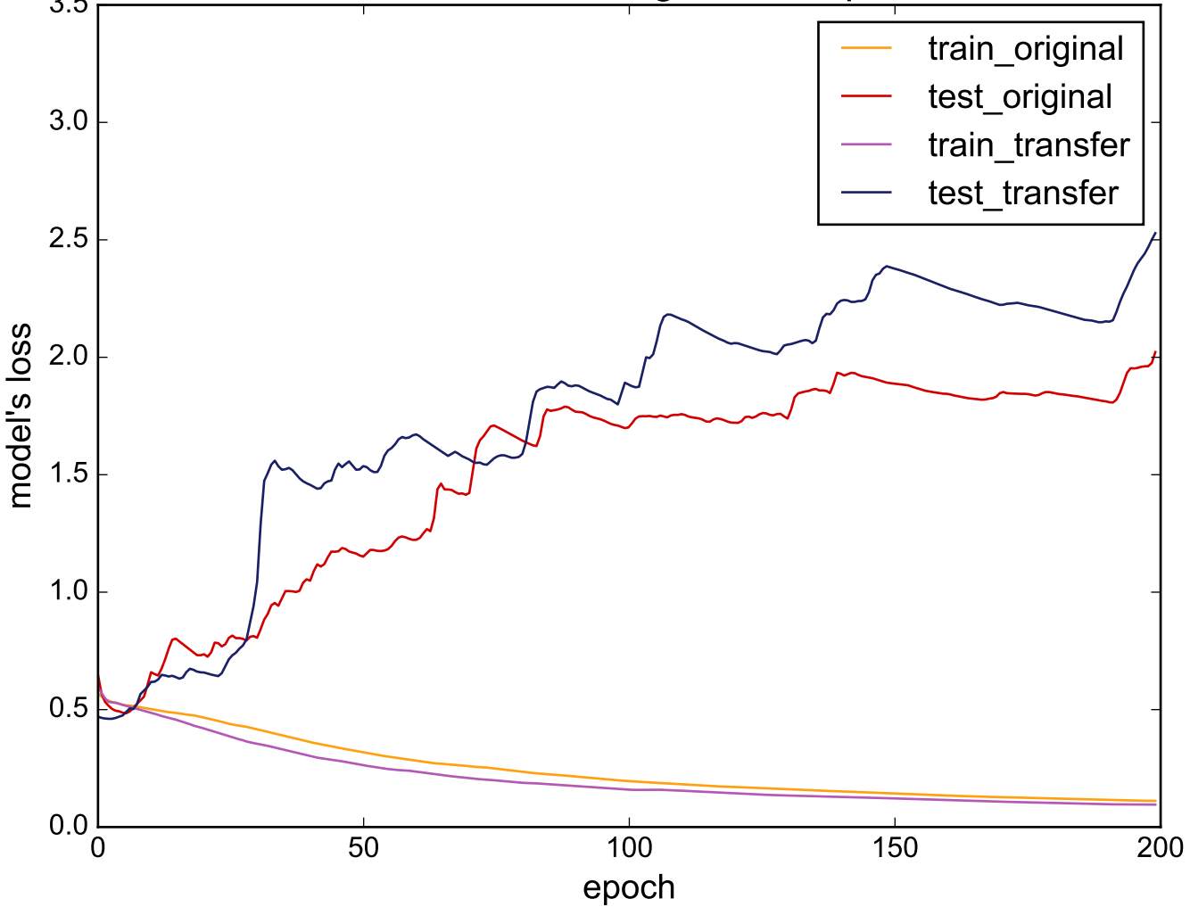
Source: Plane - Target: Earthquakes
