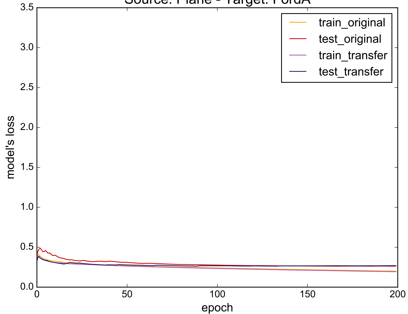
Source: Plane - Target: FordA
