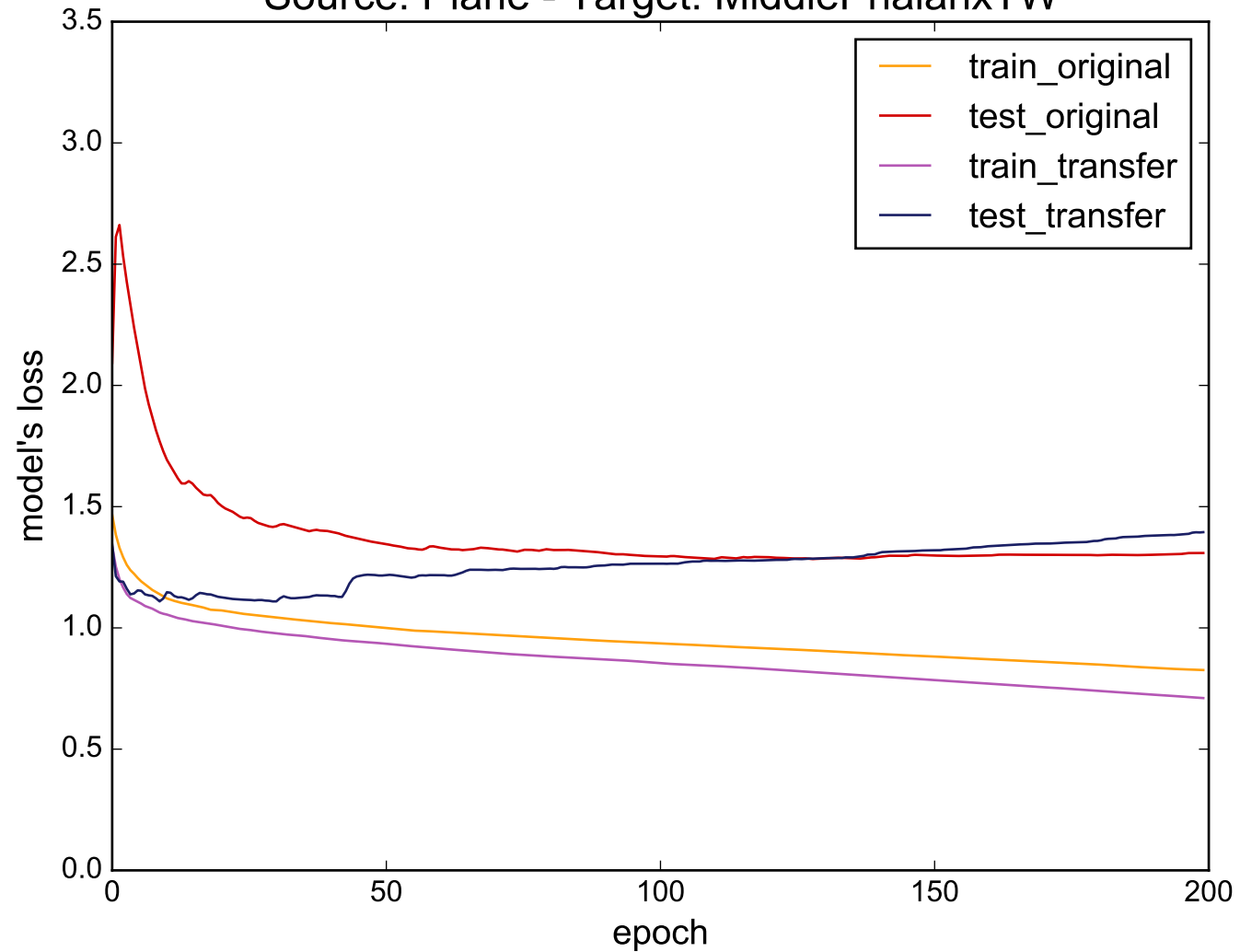
Source: Plane - Target: MiddlePhalanxTW
