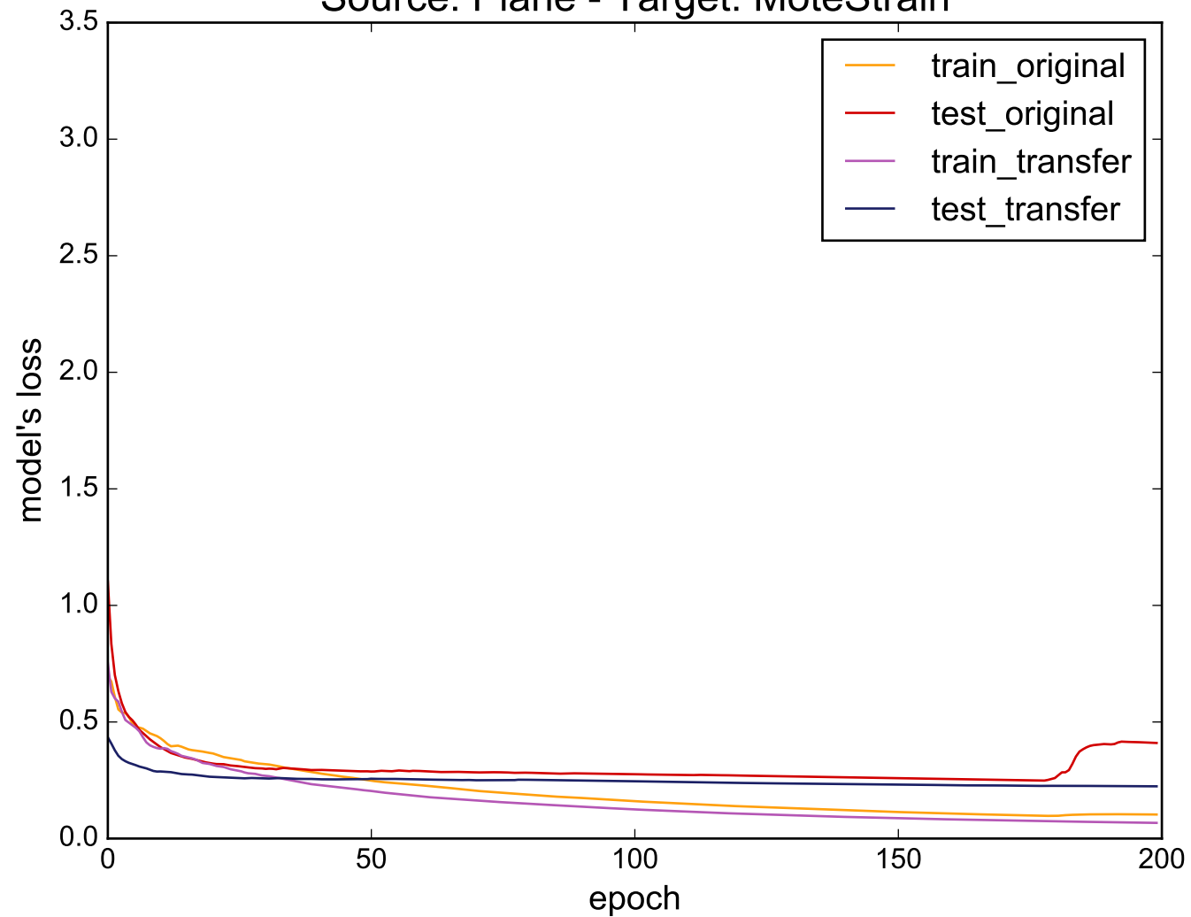
Source: Plane - Target: MoteStrain
