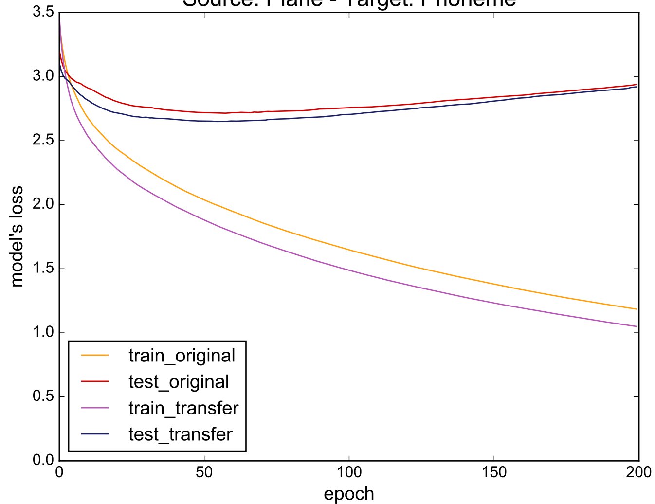
Source: Plane - Target: Phoneme
