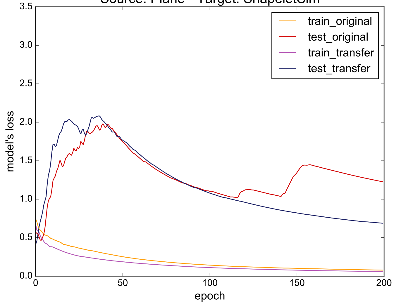
Source: Plane - Target: ShapeletSim
