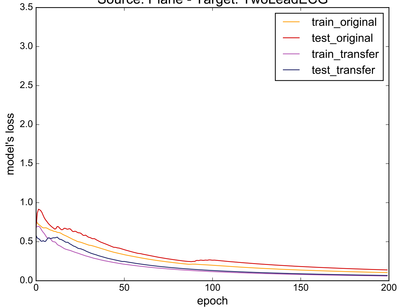
Source: Plane - Target: TwoLeadECG
