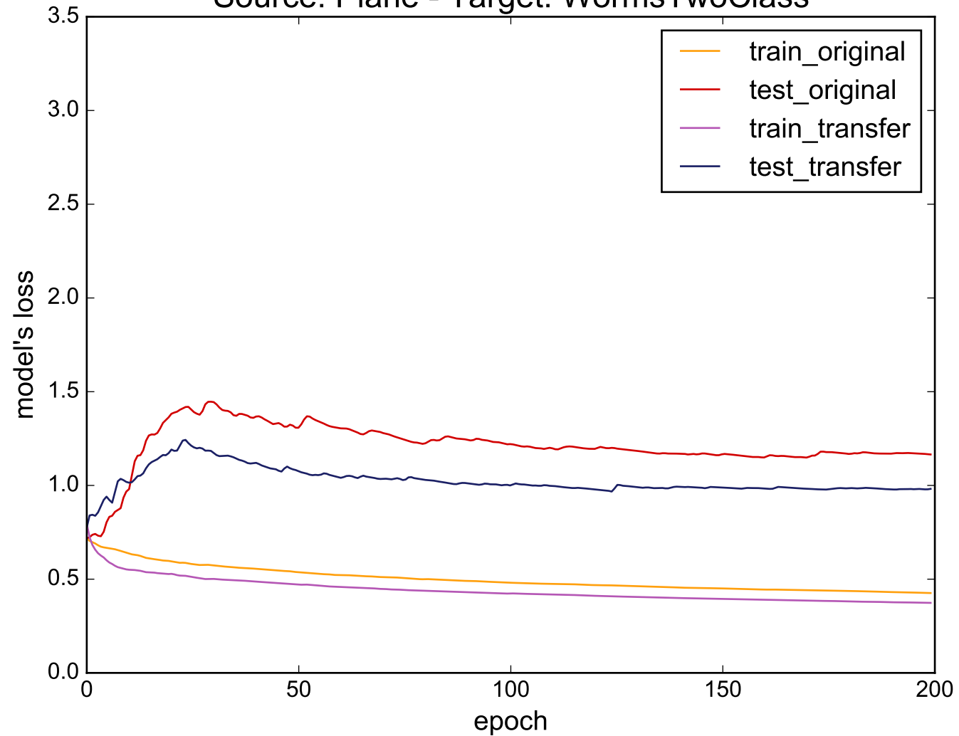
Source: Plane - Target: WormsTwoClass
