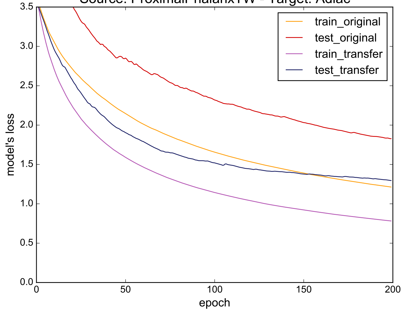
Source: ProximalPhalanxTW - Target: Adiac
