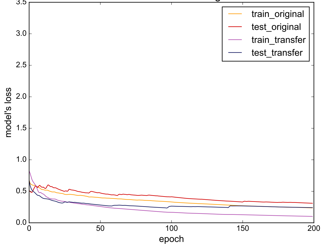
Source: ProximalPhalanxTW - Target: BirdChicken
