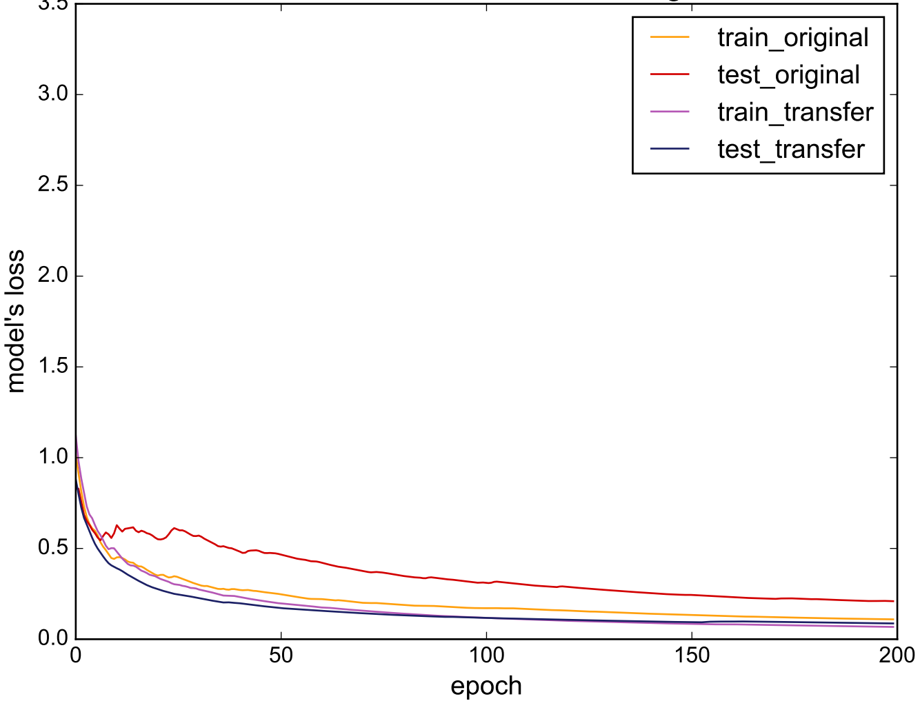
Source: ProximalPhalanxTW - Target: CBF
