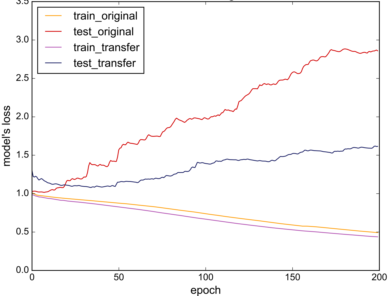
Source: ProximalPhalanxTW - Target: ChlorineConcentration
