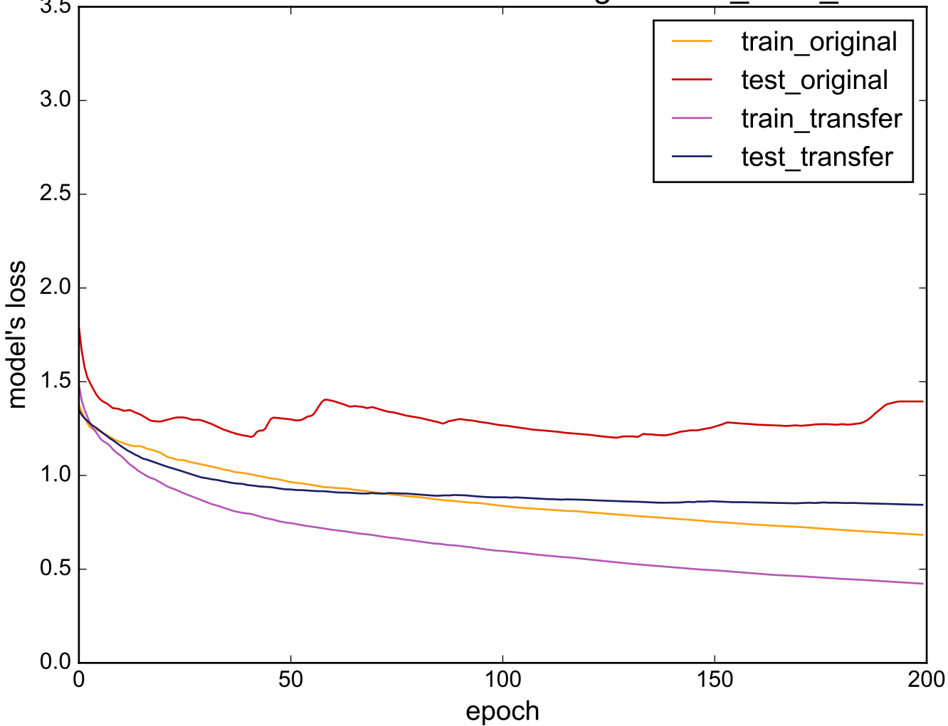
Source: ProximalPhalanxTW - Target: CinC_ECG_torso
