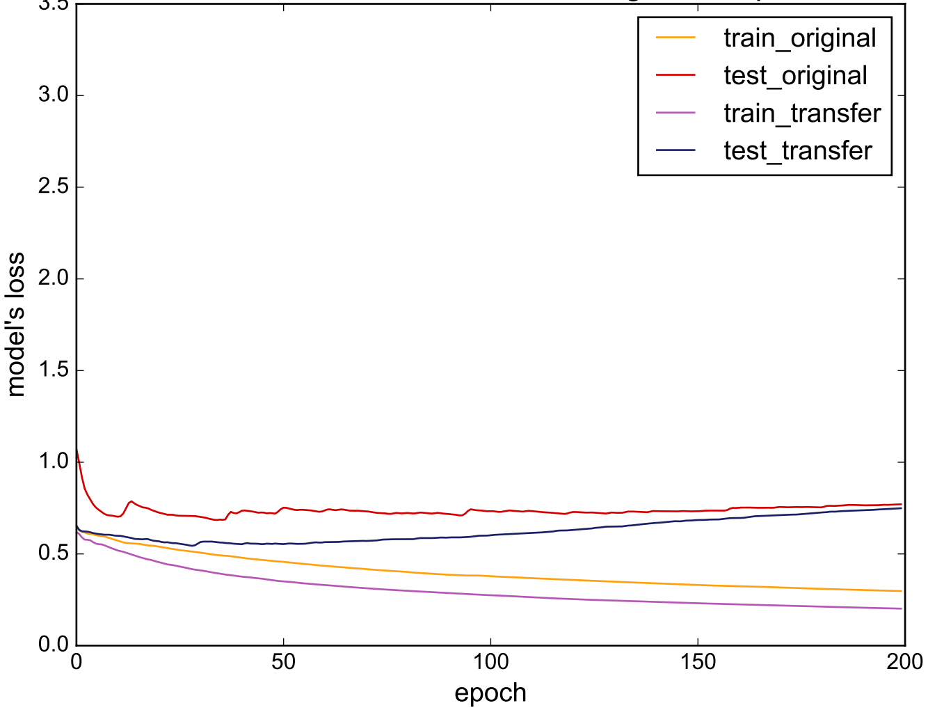
Source: ProximalPhalanxTW - Target: Computers
