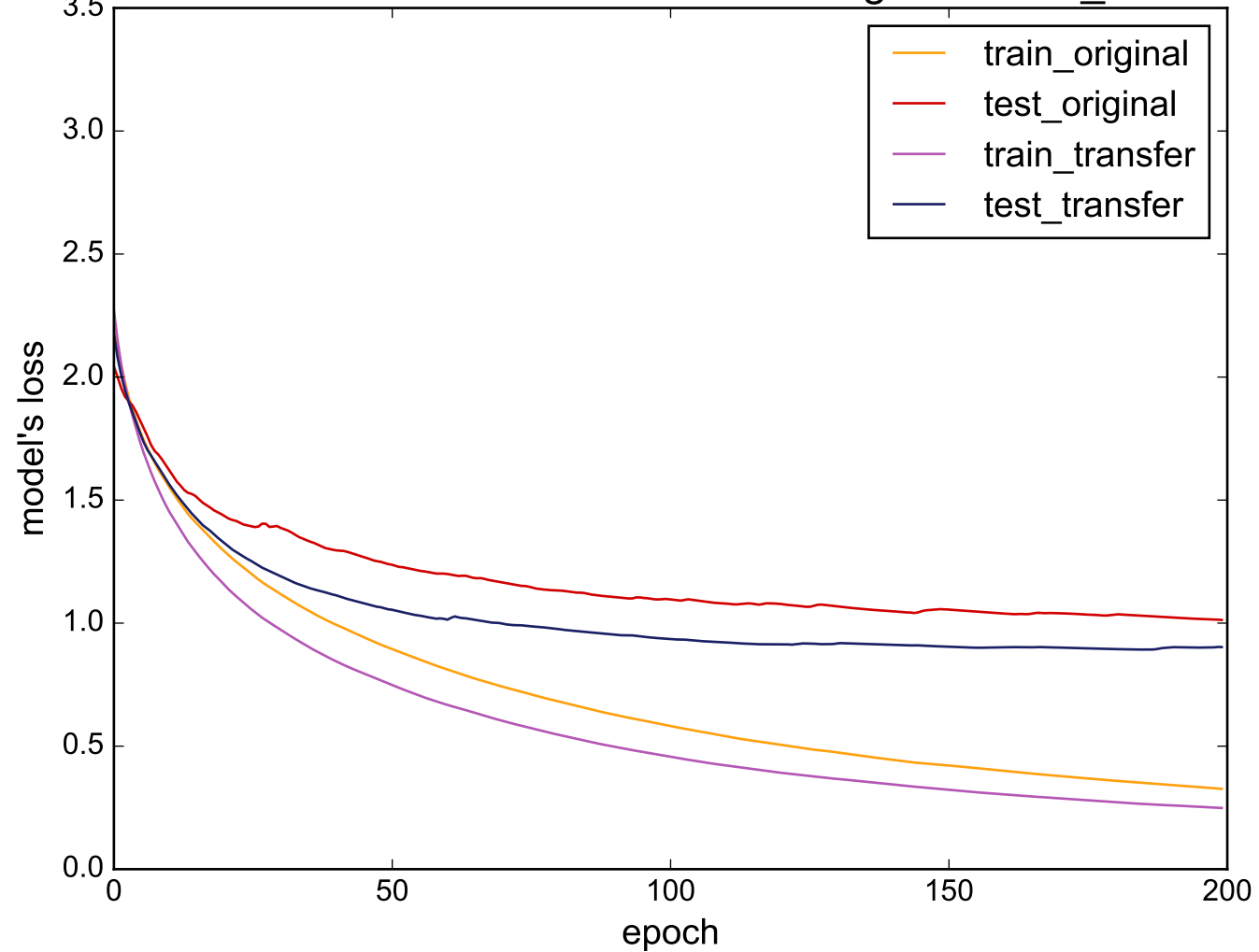
Source: ProximalPhalanxTW - Target: Cricket_X
