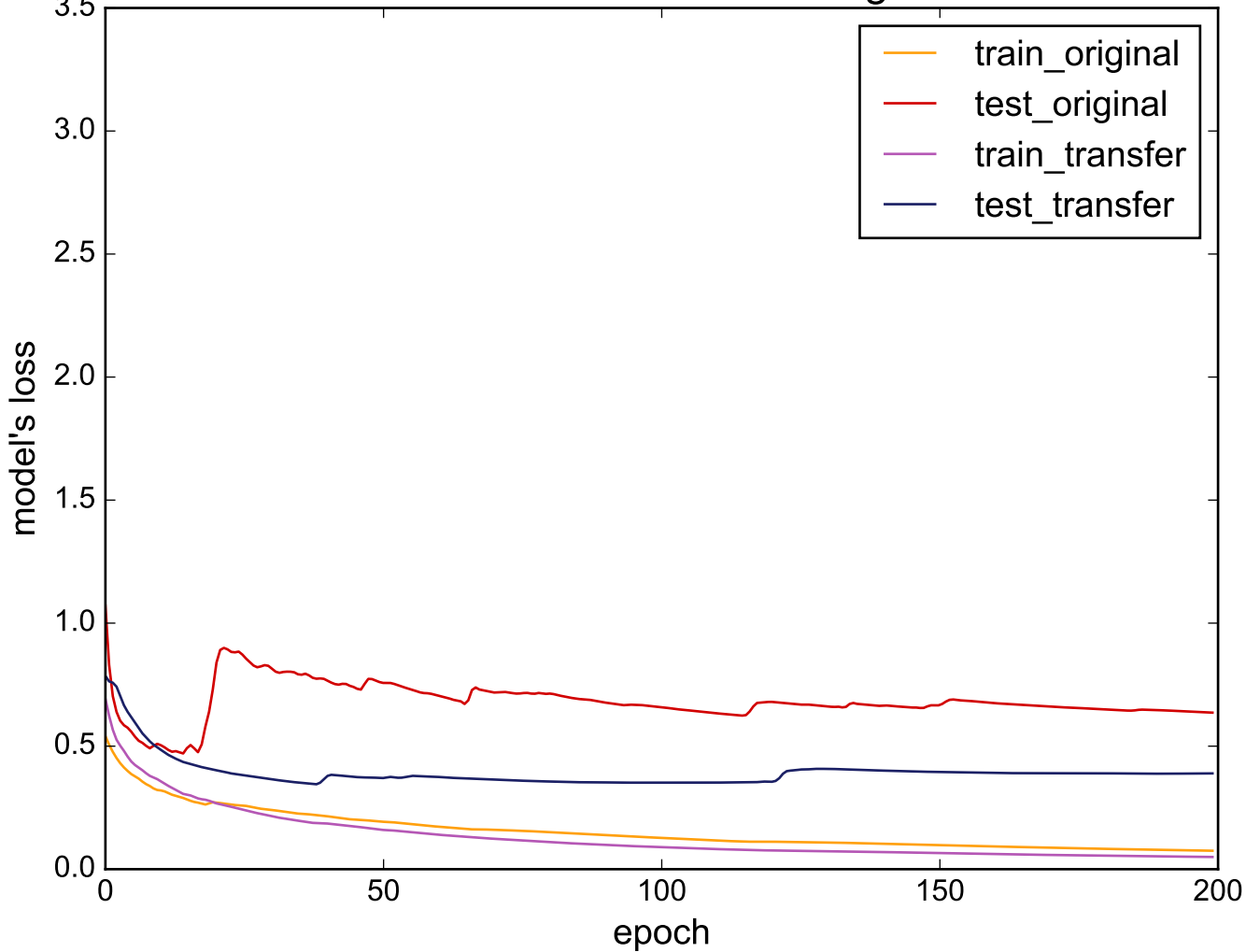
Source: ProximalPhalanxTW - Target: ECG200
