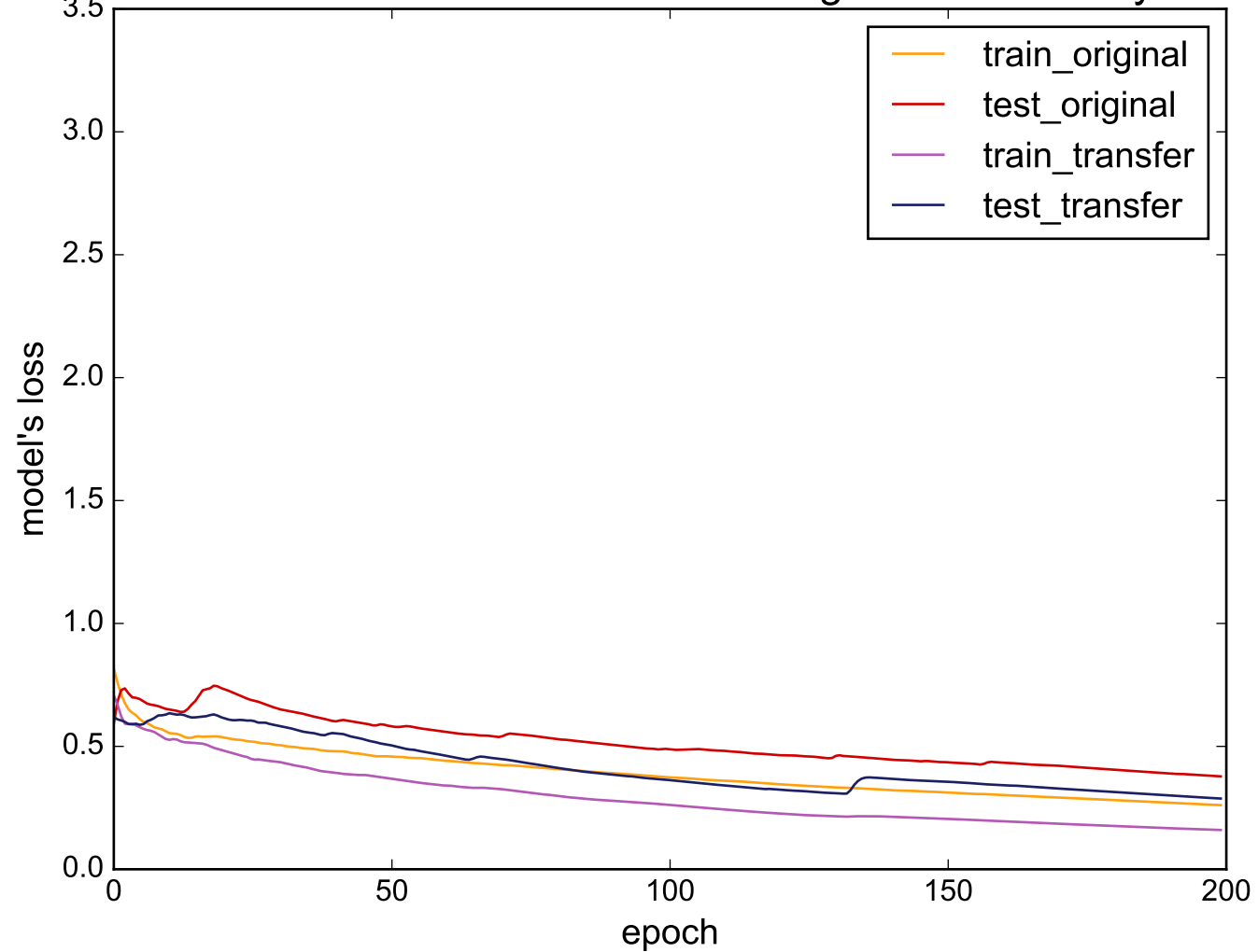
Source: ProximalPhalanxTW - Target: ECGFiveDays
