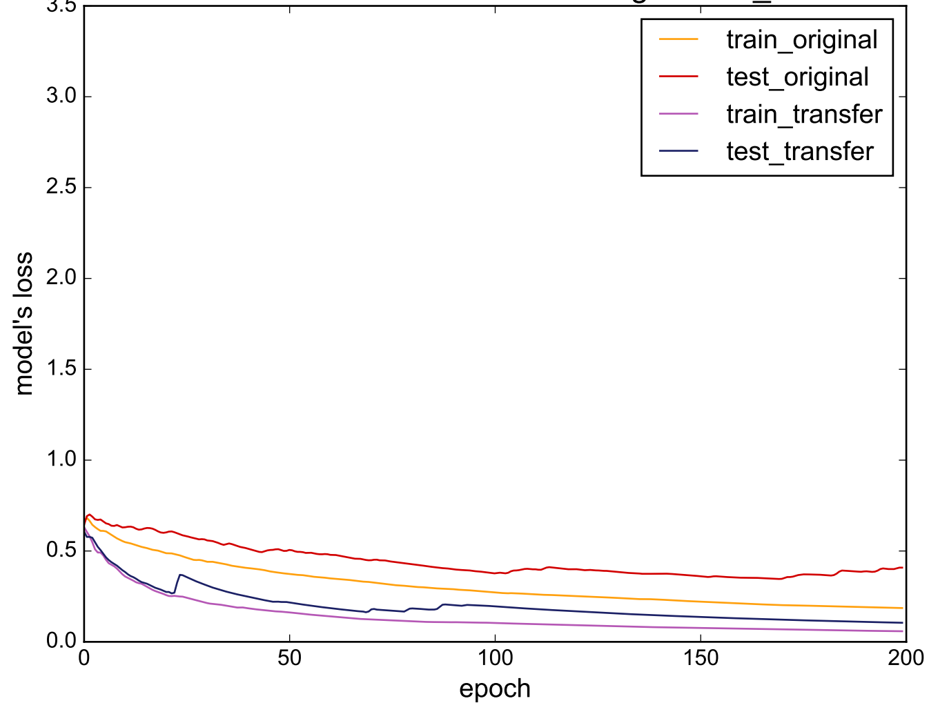
Source: ProximalPhalanxTW - Target: Gun_Point
